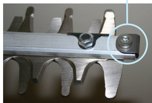
Lightweight aluminium support bar is 2mm wider than previous model and 3.5mm thicker
