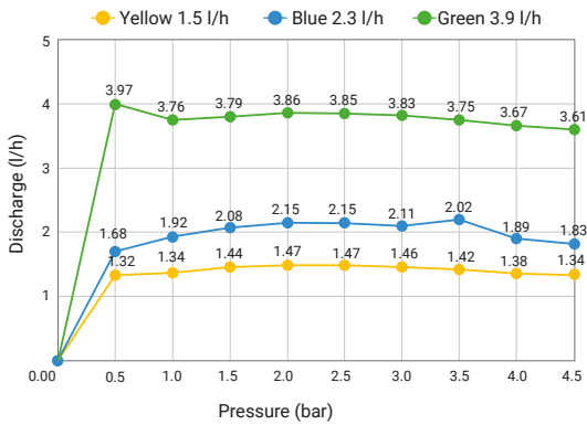
PoliDrip PC Ø20 mm 1.5 - 2.3 - 3.9 l/h
