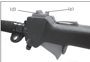
Fig 3 - Set the ignition switch (d) to the START (I) position. (e) is the throttle lock button.
